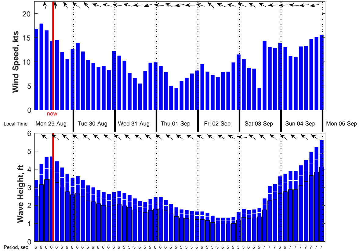
Wind & Wave Forecast for TABS Buoy X from 29-Aug-2022 01:00:00 to 04-Sep-2022 22:00:00
